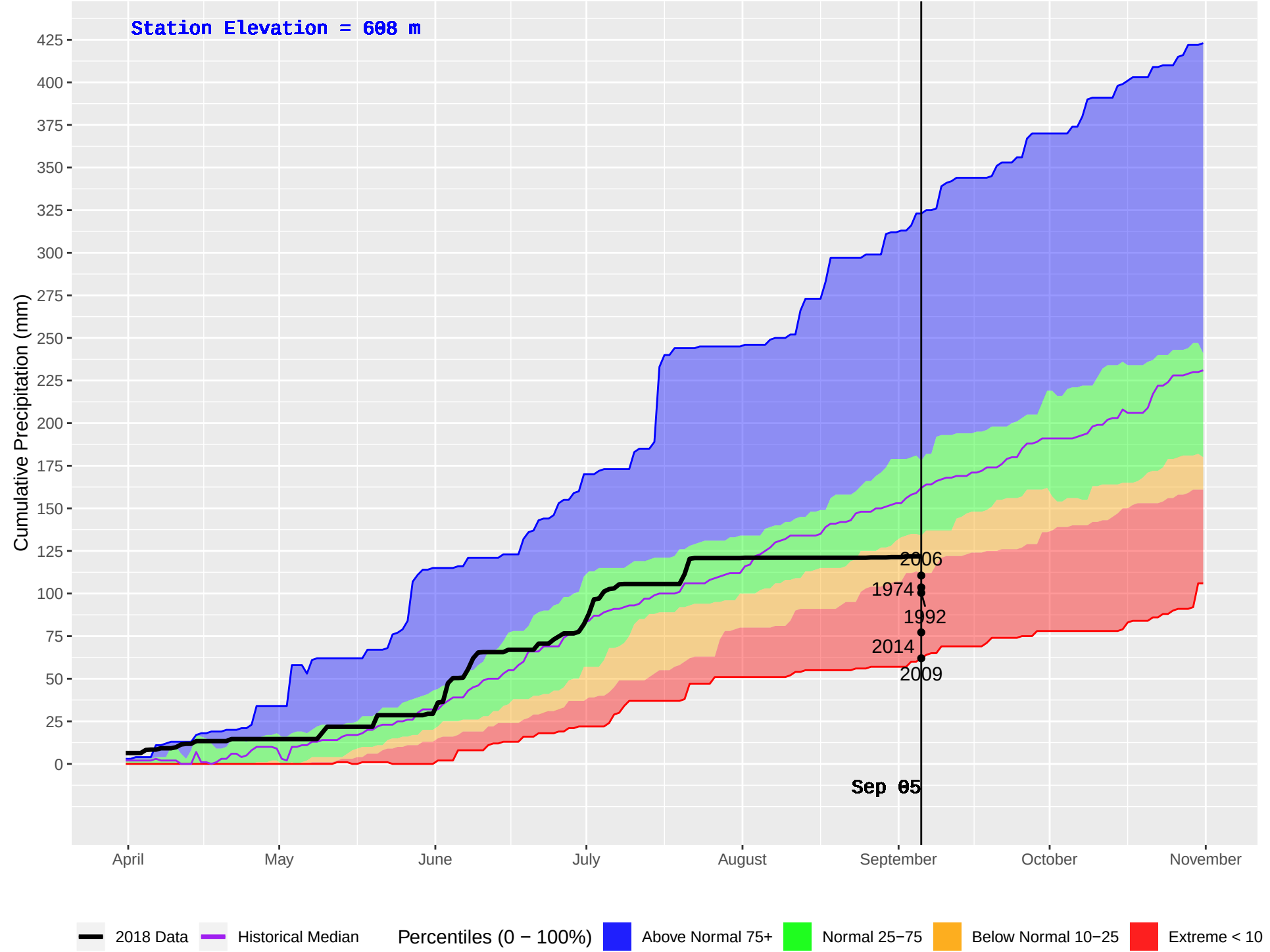
HOUSTON(DUNGATE) (162) : Historical (1974–2016) and Current (2018) Daily Cumulative Precipitation
