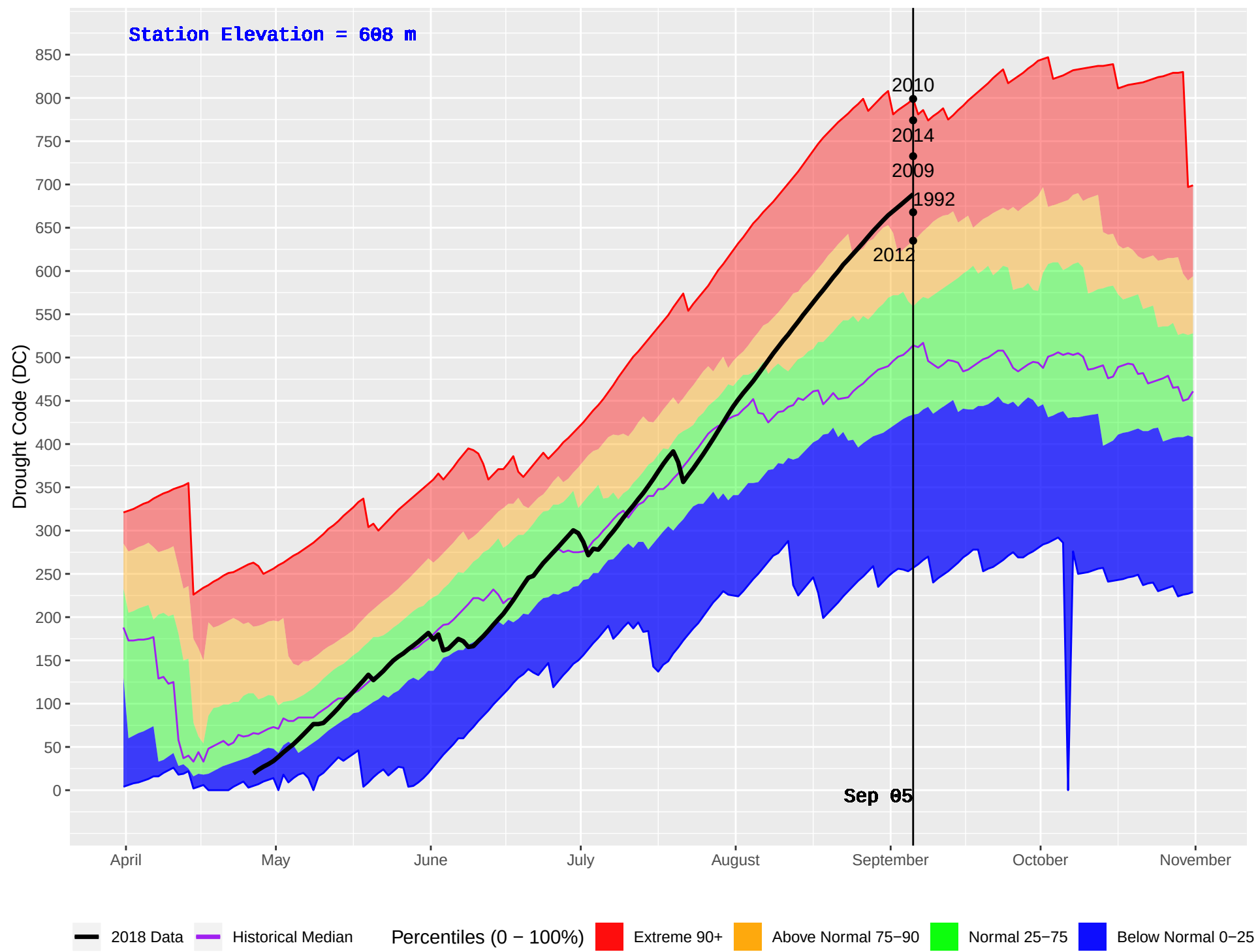
HOUSTON(DUNGATE) (162) : Historical (1974–2016) and Current (2018) Daily Drought Code (DC)
