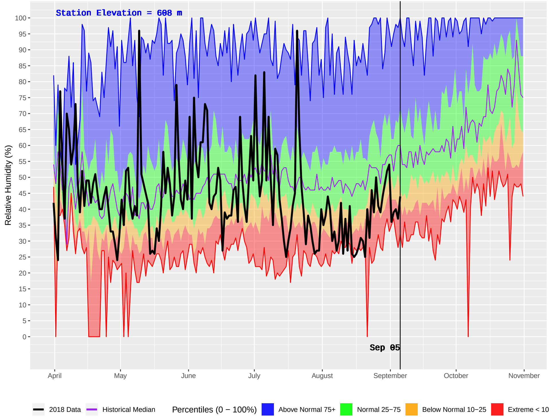
HOUSTON(DUNGATE) (162) : Historical (1974–2016) and Current (2018) Daily Relative Humidity
