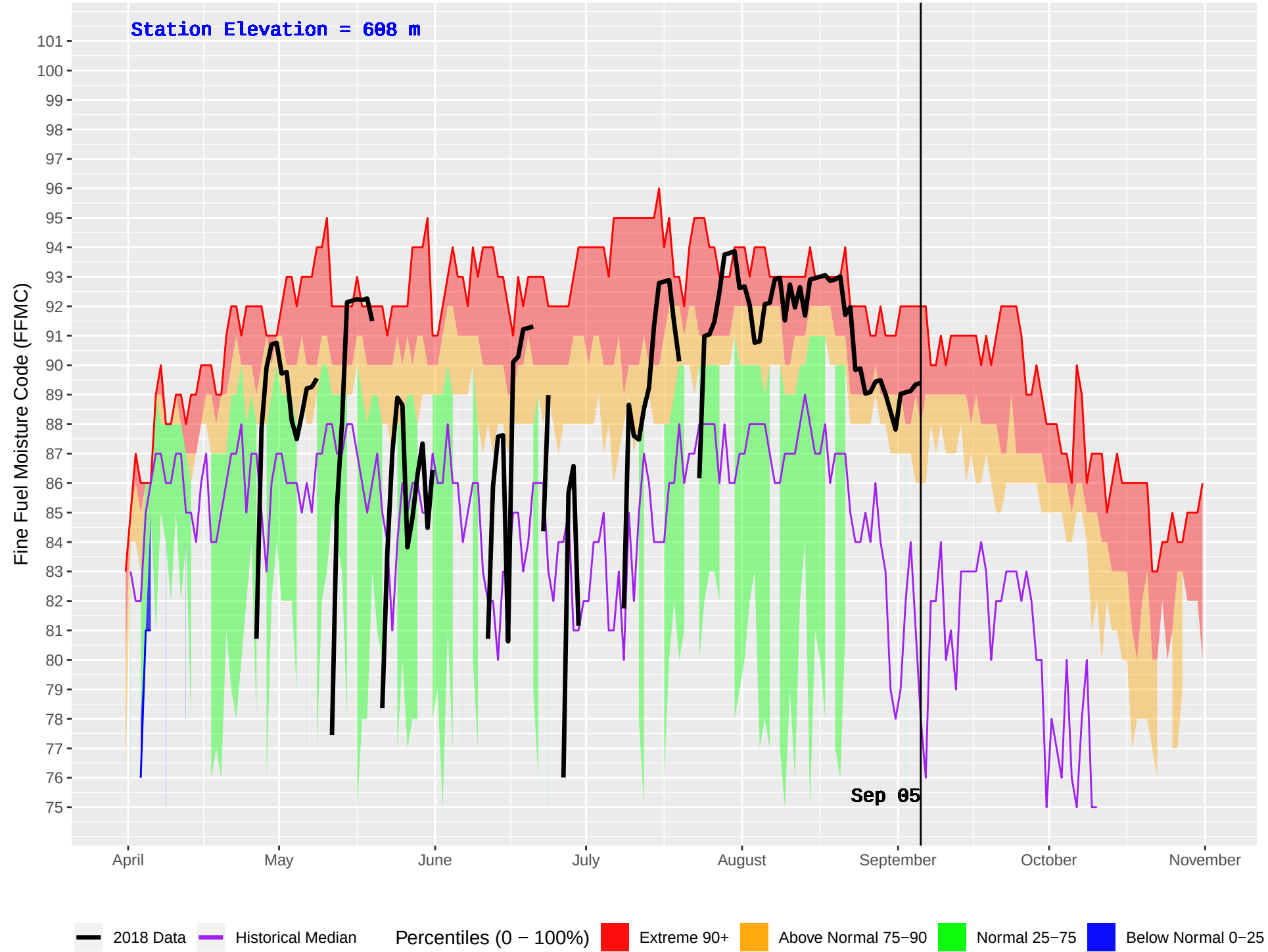
HOUSTON(DUNGATE) (162) : Historical (1974–2016) and Current (2018) Daily Fine Fuel Moisture Code (FFMC)
