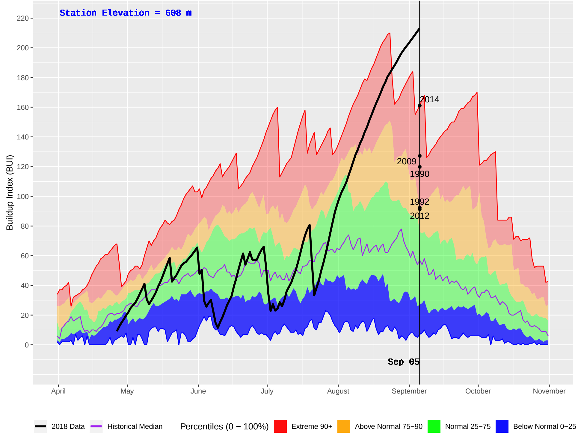
HOUSTON(DUNGATE) (162) : Historical (1974–2016) and Current (2018) Daily Buildup Index (BUI)
