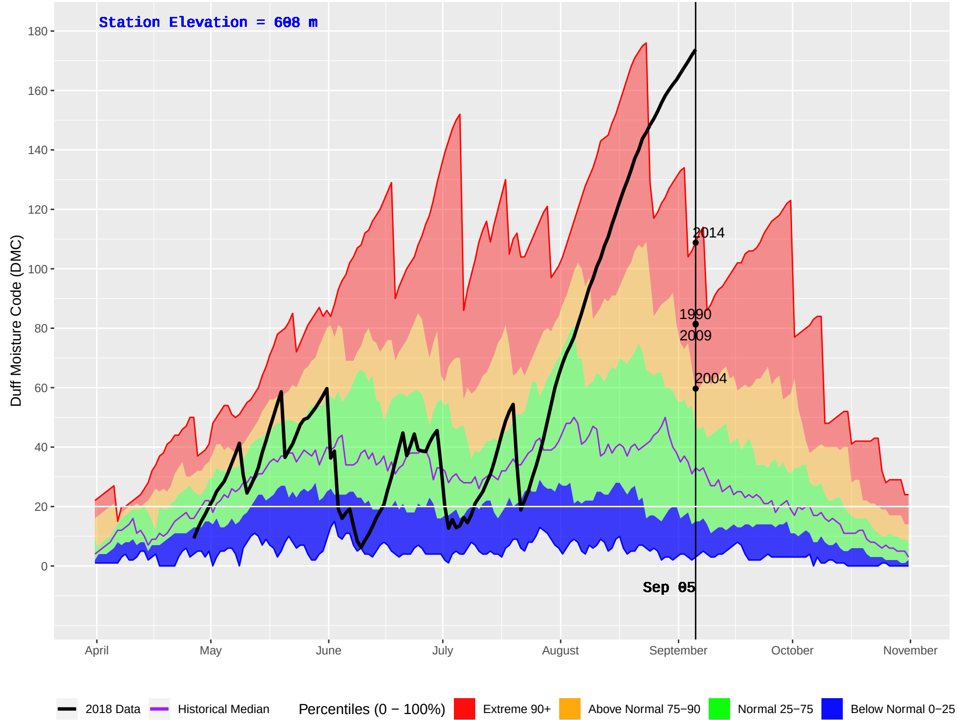
HOUSTON(DUNGATE) (162) : Historical (1974–2016) and Current (2018) Daily Duff Moisture Code (DMC)
